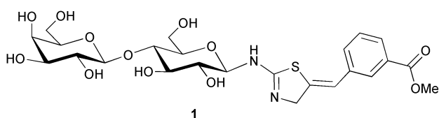
Fig. 1 Structure of monovalent lactoside 1 .
