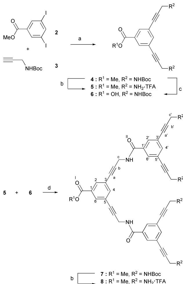
Scheme 1 Reaction conditions: a) Pd(o), CuI, NEt 3 , CH 3 CN, 2 d (65%); b) TFA, CH 2 Cl 2 , 20 min (quant.); c) Tesser's base, 14 h (quant.); d) BOP, i Pr 2 NEt, CH 3 CN, 14 h (71%).
